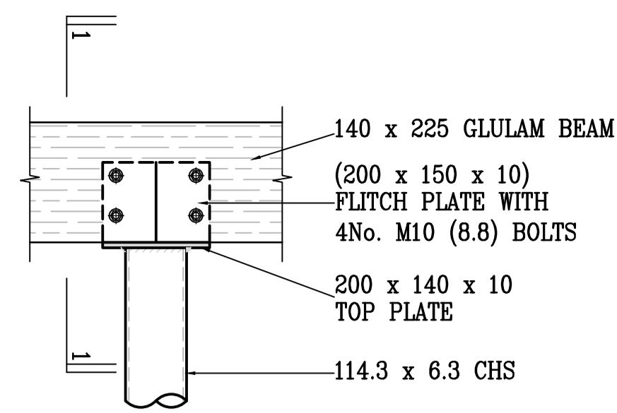
DETAIL 1 1:10
