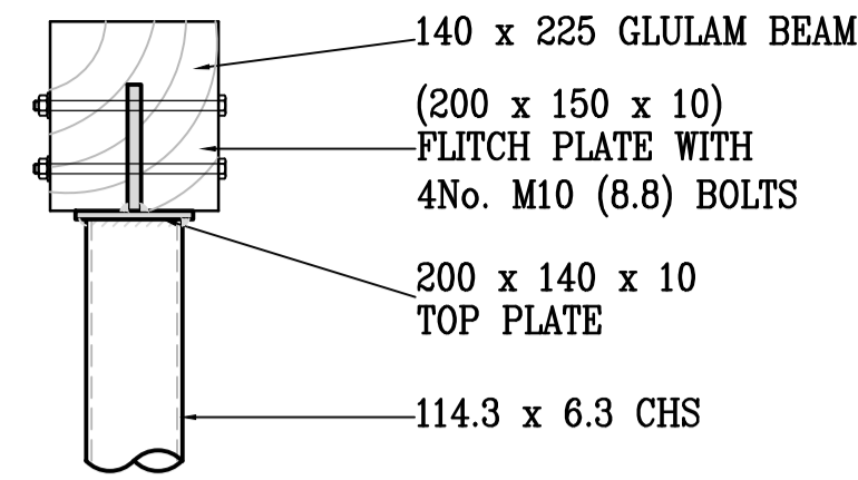
SECTION 1 - 1 1:10
