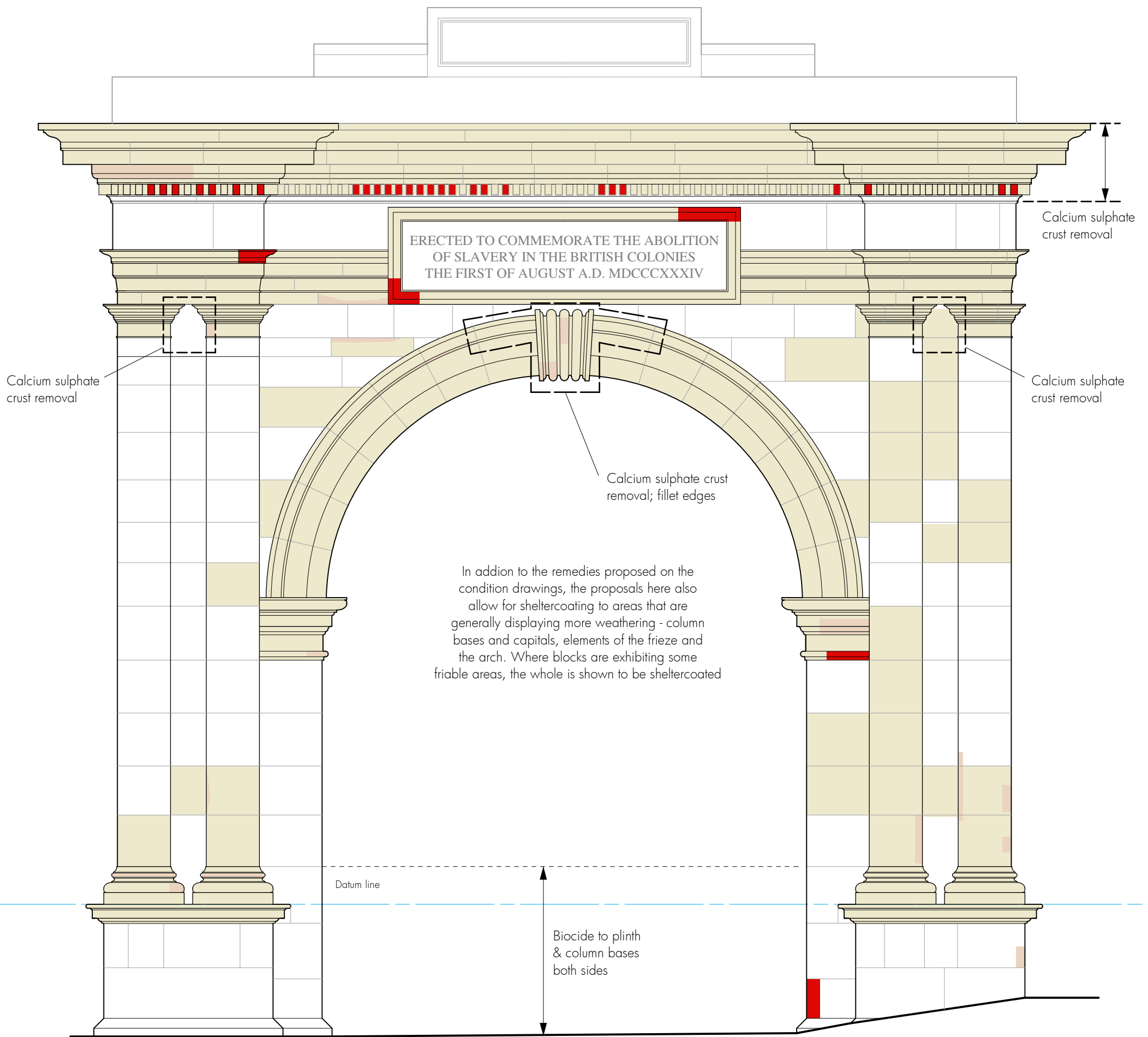
South east elevation (facing Farmhill Lane)
