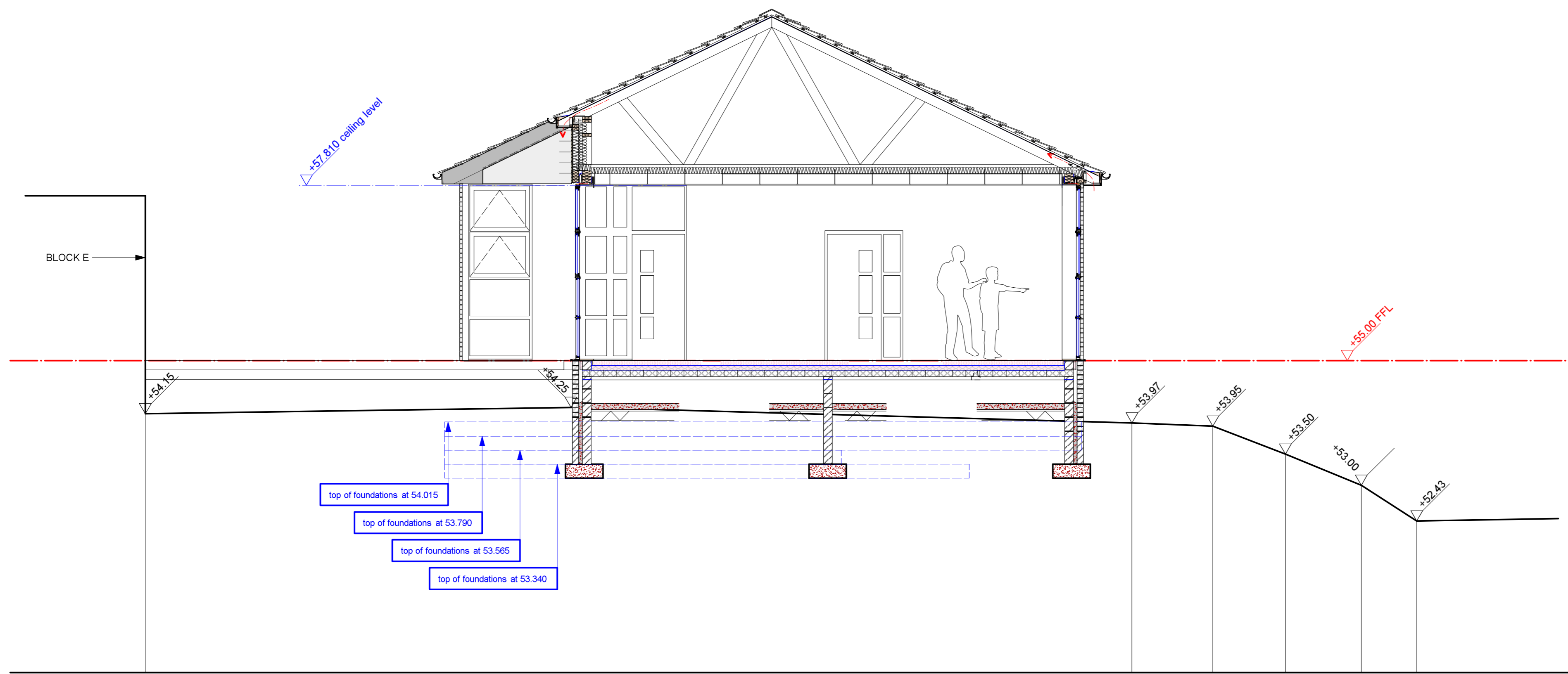
SECTION 4 scale 1:50
