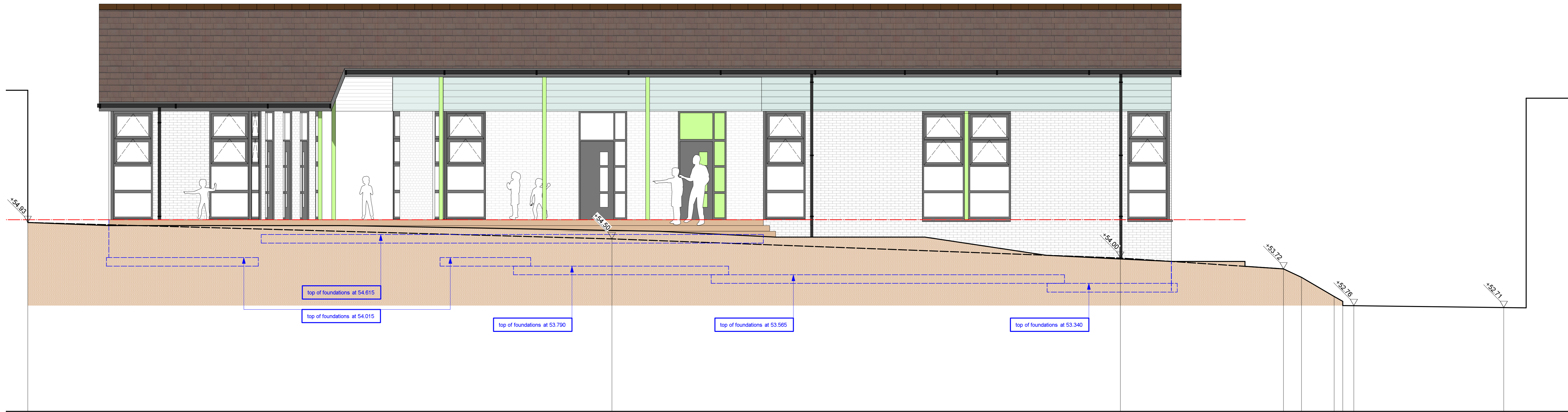
SECTION 1 scale 1:50
