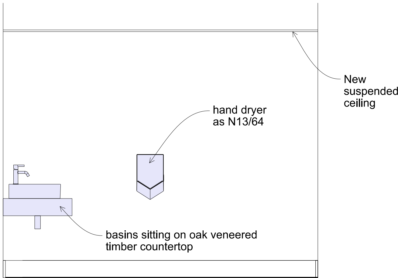
Proposed Elevation E3
