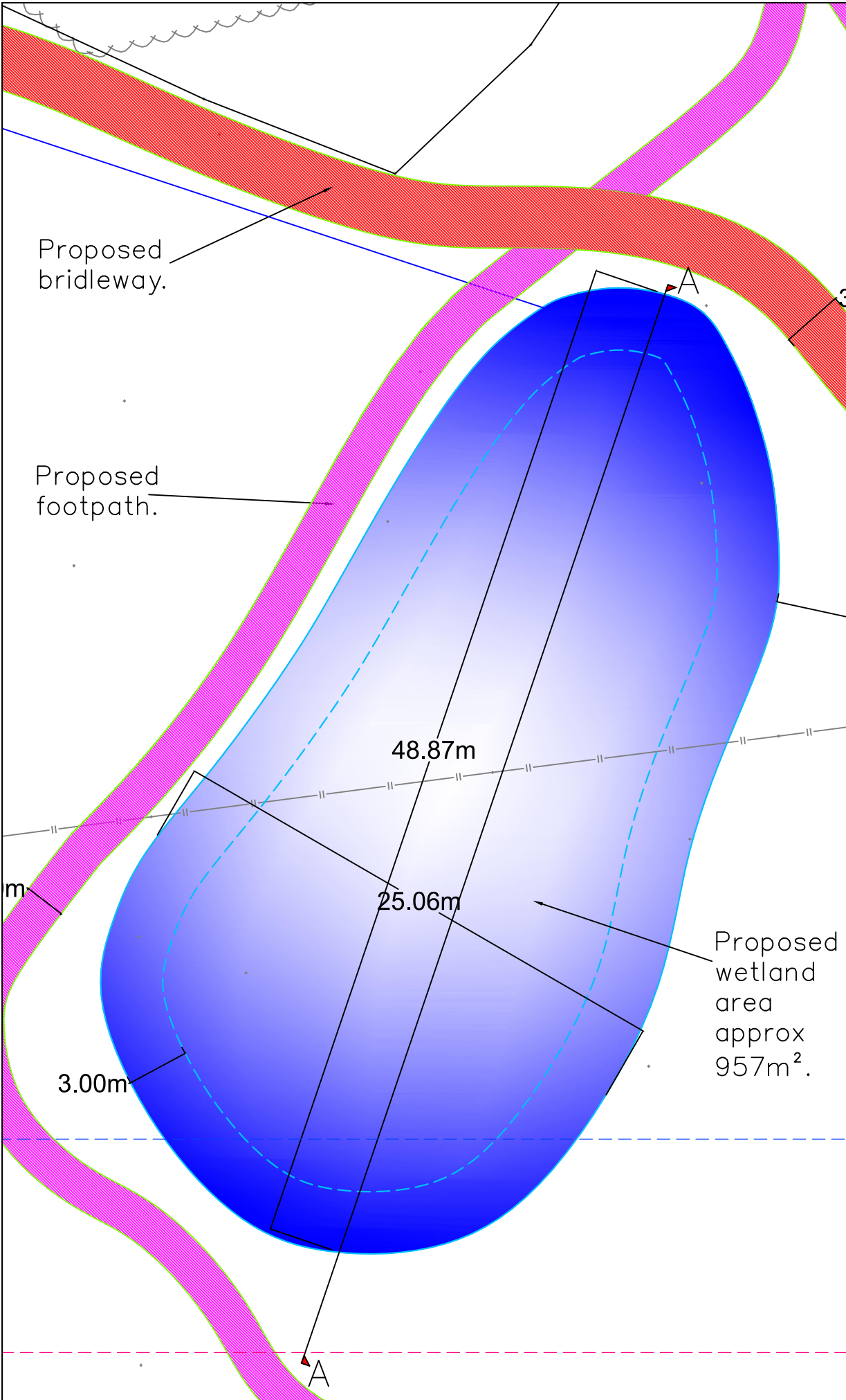
Proposed Wetland Plan Scale 1/250
