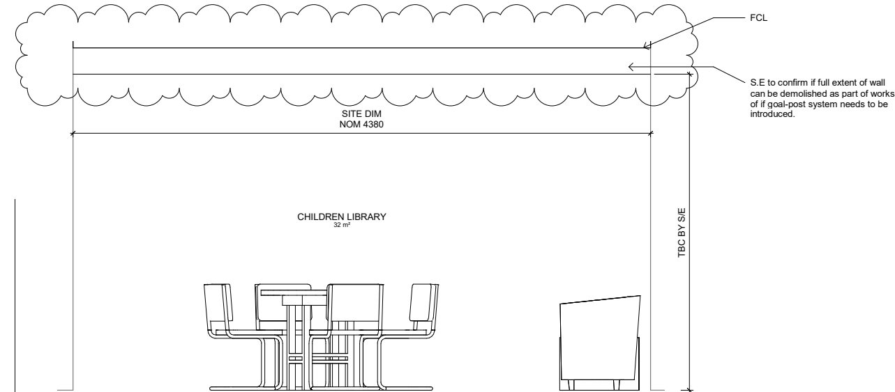
Elevation Three 1 : 20
