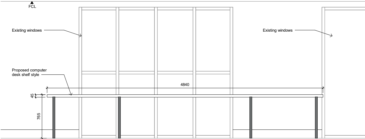
Elevation Four 1 : 20
