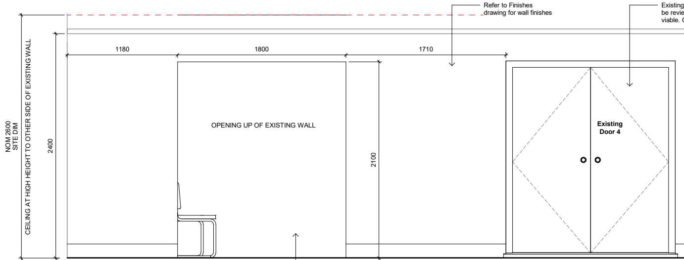
Elevation Two 1 : 20
