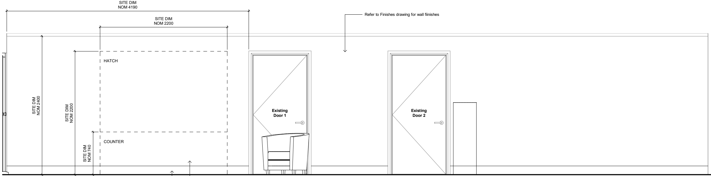
Elevation One 1 : 20
