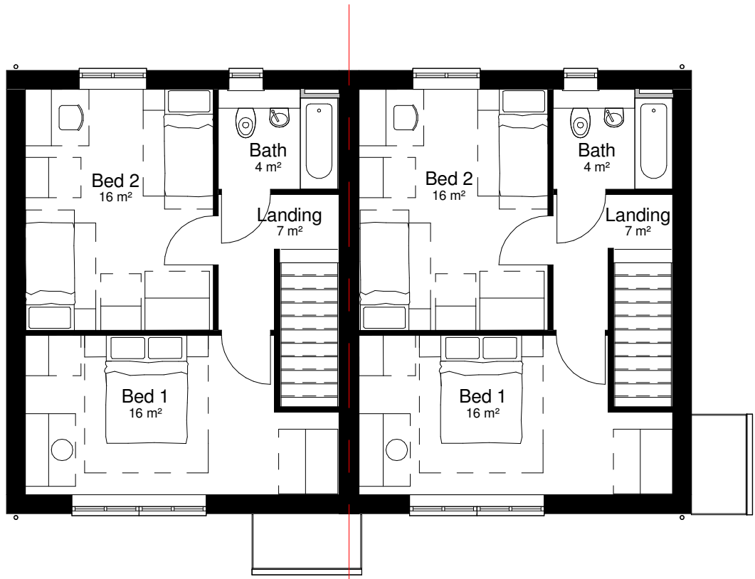
First Floor 1 : 100
