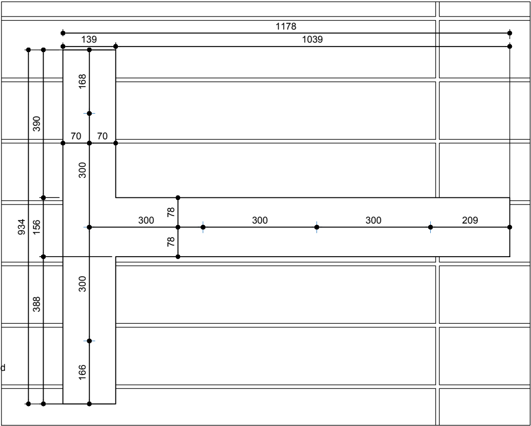
LETTER FIXING POINT ELEVATION @1:10
