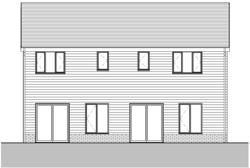
Rear Elevation 1 : 100
