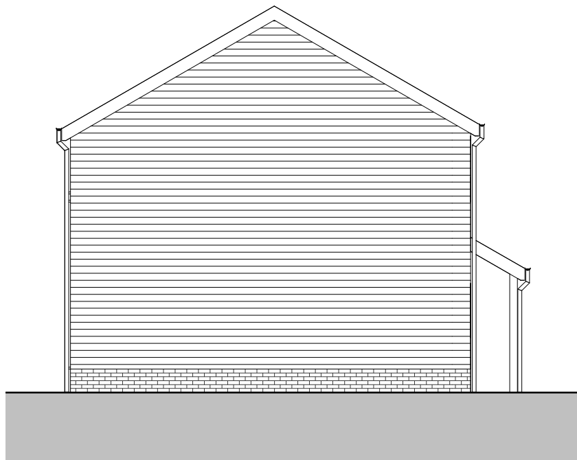
Left Elevation 1 : 100
