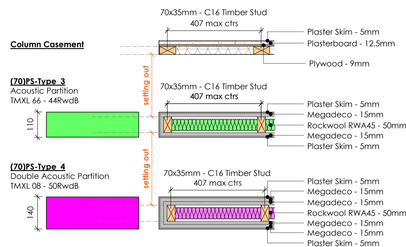
Internal Wall Types - Plaster Skim 1 : 10
