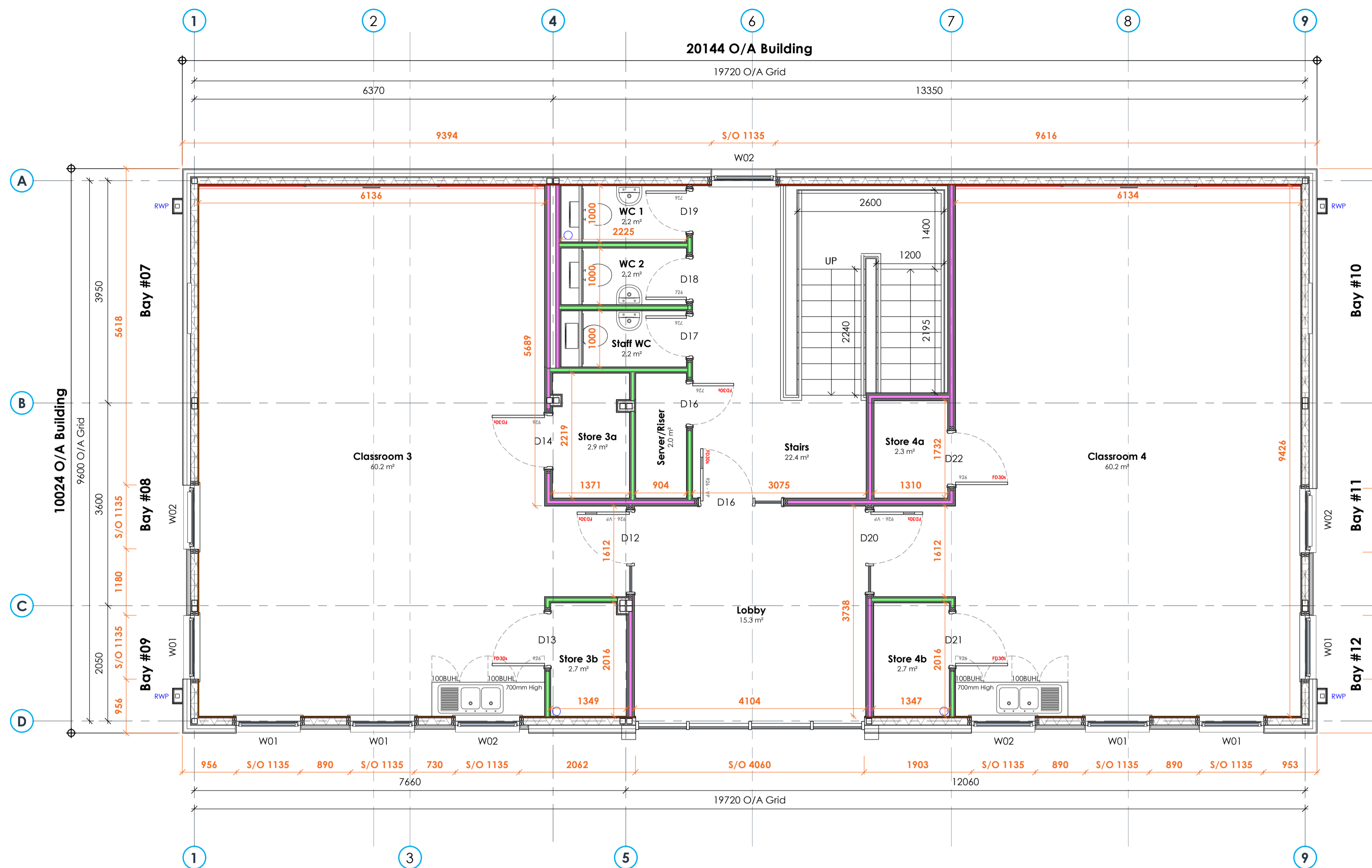
01 First Floor Plan 1 : 50
