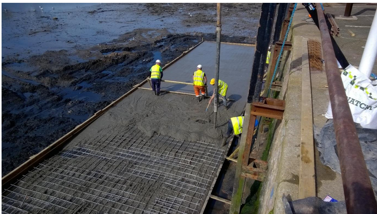
Brixham Inner harbour drying grid April 2016
