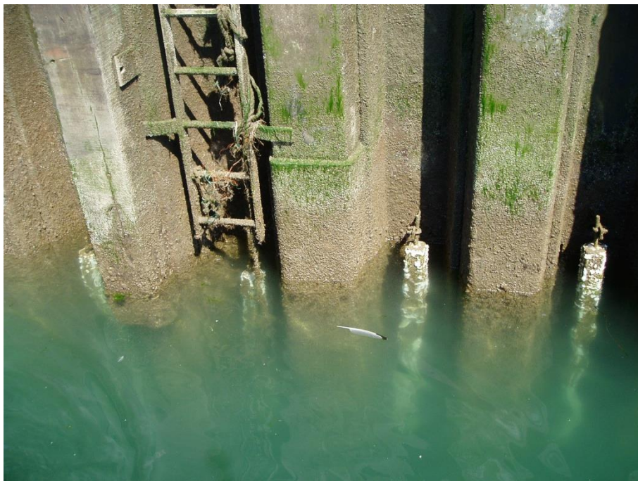
Passive CP installation and repair, Brixham Harbour, Brixham
