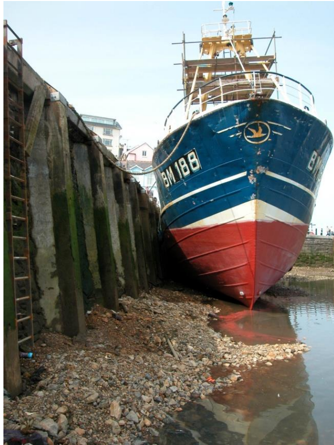
Repair of timber fenders, Crane Pier, Brixham Harbour, Brixham
