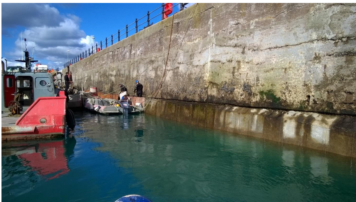
Princess Pier toe encasement Feb 2016
