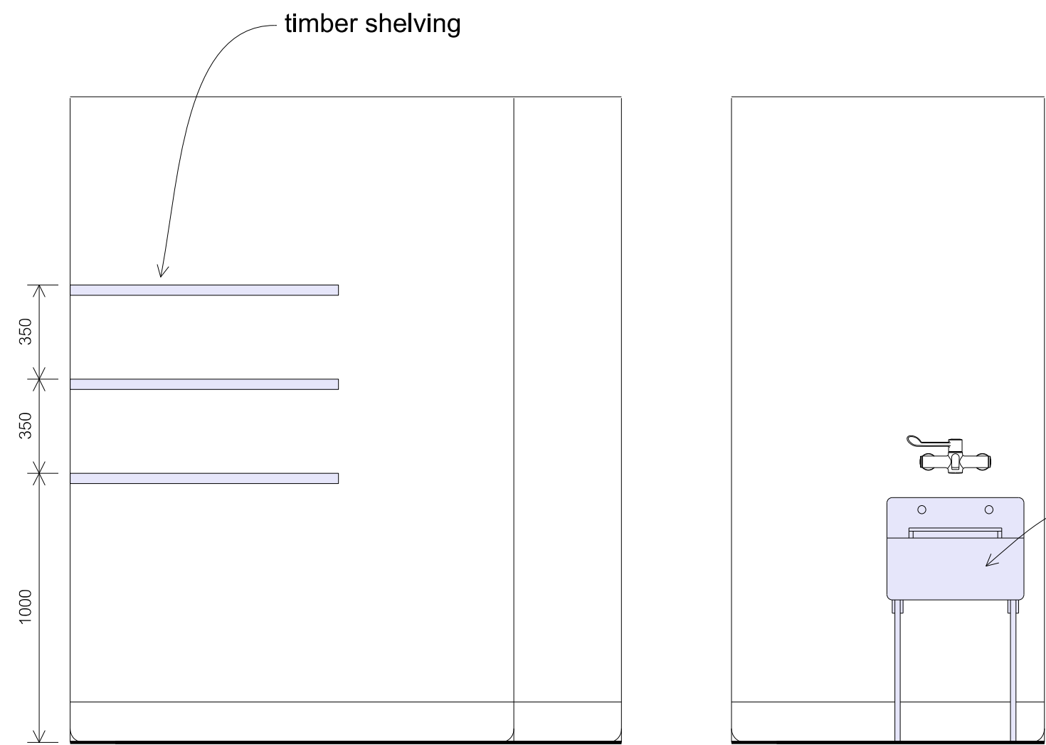
Proposed Cleaners Cupboard Elevations, Front and Side
