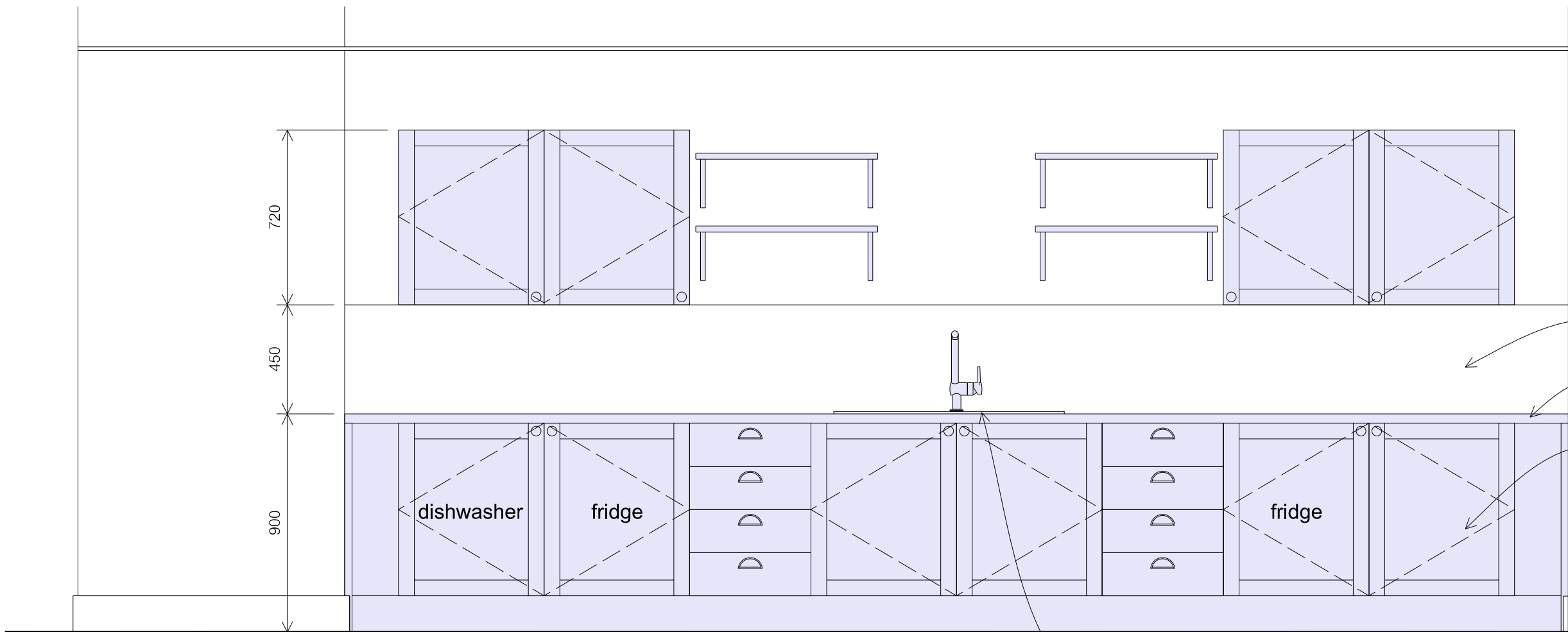
Proposed Kitchen Elevation
