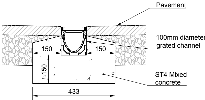
Detail 01 1:10 1104 Grated Channel Drain
