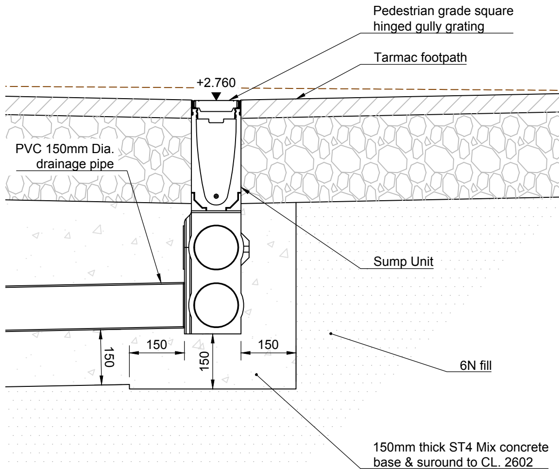
Detail 02 1:10 1104 Sump Unit
