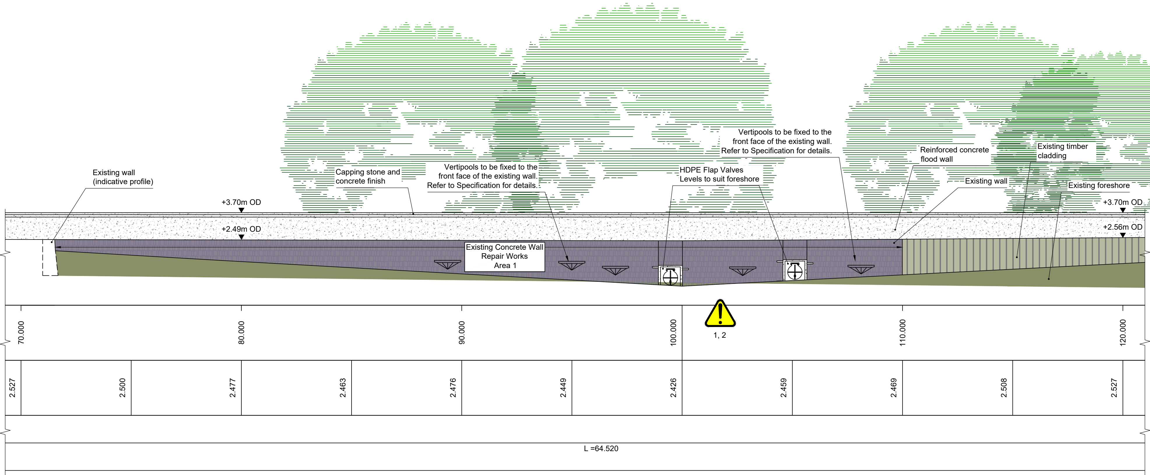
Elevation - View from Lake Side 1:100
