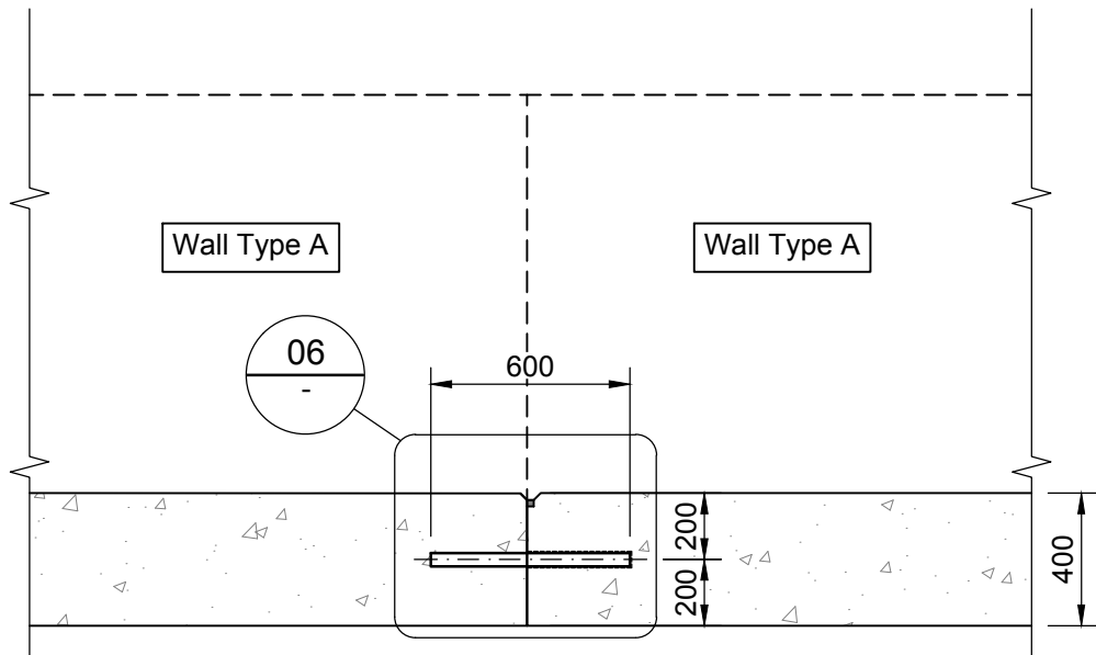
Wall Type A and Type A Connection
