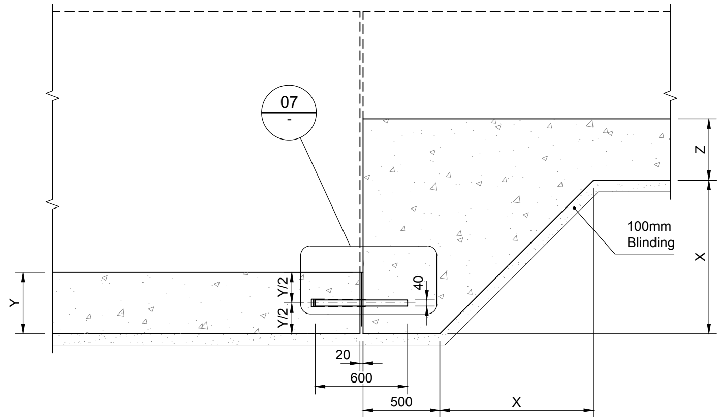
Typical Step Connection Detail
