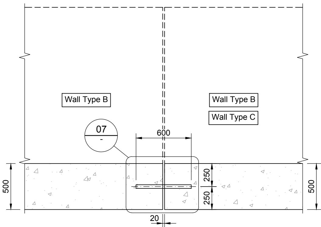
Wall Type B and Type B Wall Type B and Type C Connection
