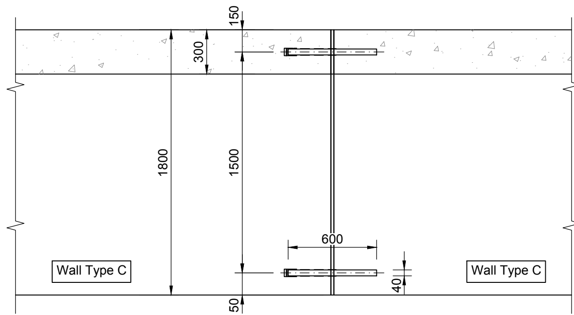
Slab Connections - Plan Views
