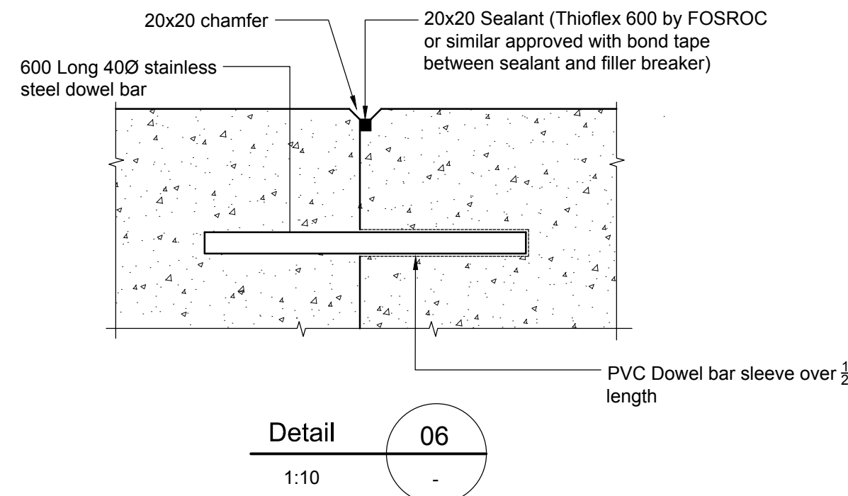
Contraction Joint (CJ) Typical
