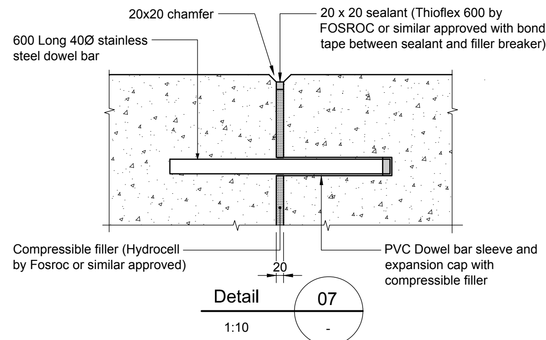
Expansion Joint (EJ) Typical
